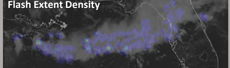
GLM gridding technique produces other gridded products under evaluation for potential AWIPS integration
