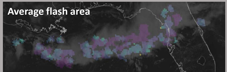
GLM gridding technique produces other gridded products under evaluation for potential AWIPS integration
