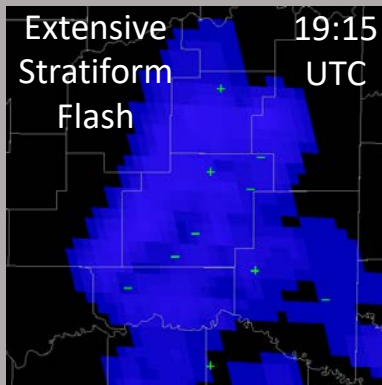
GLM gridding technique produces other gridded products under evaluation for potential AWIPS integration
