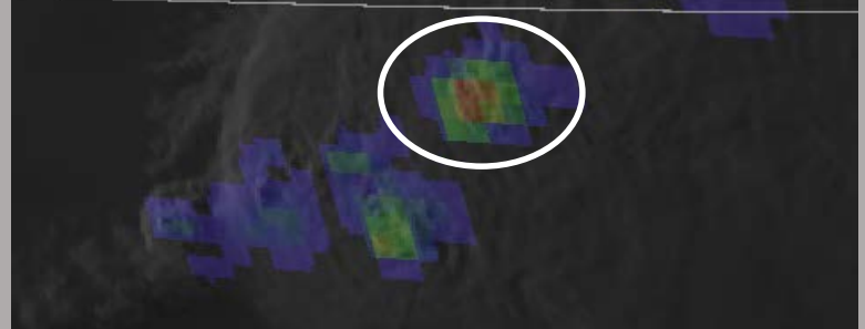
Collocation of greatest flash rates and tallest storms
