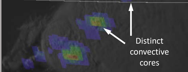
GLM FED with visible imagery from an ABI mesoscale sector
